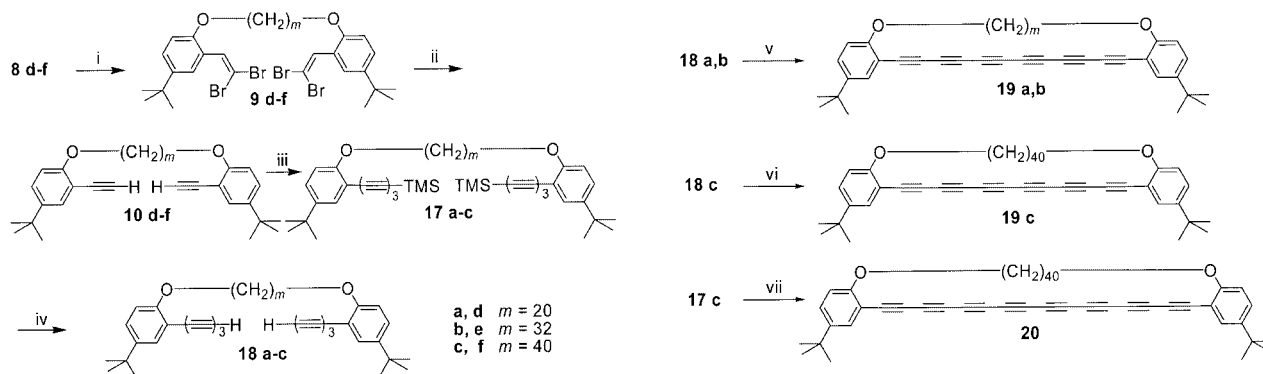
Scheme 4. Synthesis of macrocyclic \alpha,\omega -diphenylhexaynes 19a–c and octayne 20 . i) \text{PPh}_3 , \text{CBr}_4 , \text{CH}_2\text{Cl}_2 ; ii) \text{LDA} , -80^\circ\text{C} ; iii) \text{Br}-\text{C}\equiv\text{C}-\text{C}\equiv\text{C}-\text{TMS} ( 16 ), \text{BuLi} , \text{THF} , 0^\circ\text{C} ; \text{CuCl} , pyridine; iv) \text{K}_2\text{CO}_3 , \text{MeOH} , \text{THF} ; v) \text{TMEDA} , \text{CuCl} , \text{O}_2 , acetone; vi) [\text{Pd}(\text{PPh}_3)_2\text{Cl}_2] , \text{CuI} , \text{NEt}_3 , \text{CH}_2\text{Cl}_2 , 0^\circ\text{C} ; \text{Br}-\text{C}\equiv\text{C}-\text{C}\equiv\text{C}-\text{TMS} ( 16 ) (diluted, 3 mmol); vii) \text{K}_2\text{CO}_3 , [\text{Pd}(\text{PPh}_3)_2\text{Cl}_2] , \text{CuI} , \text{NEt}_3 , \text{CH}_2\text{Cl}_2 , 0^\circ\text{C} , \text{Br}-\text{C}\equiv\text{C}-\text{C}\equiv\text{C}-\text{TMS} ( 16 ) (concentrated, 30 mmol). Yields: 19a (33%), 19b (18%), 19c (58%), and 20 (1.1%).
