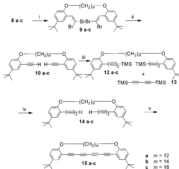
Scheme 3. Synthesis of the macrocyclic \alpha,\omega -diphenyltetraynes 15a–c . i) PPh_3 , CBr_4 , CH_2Cl_2 ; ii) LDA, -80^\circ C ; iii) excess of H-C\equiv C-TMS ( 11 ), TMEDA, CuCl , O_2 , acetone; iv) K_2CO_3 , MeOH, THF; v) TMEDA, CuCl , O_2 , acetone, high dilution. Yields: 15a (7%), 15b (8%) and 15c (1.3%).
