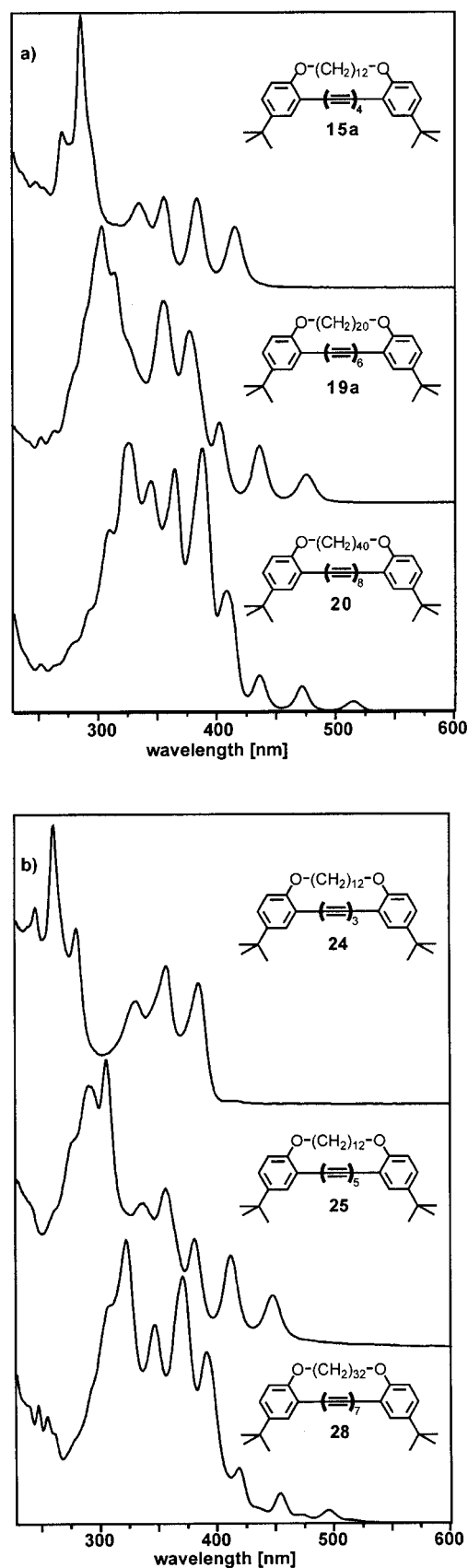
Figure 3. Comparative UV/Vis spectra of a) the tetrayne 15a , hexayne 19a and octayne macrocycle 20 , and b) the triyne 24 , pentayne 25 and heptayne macrocycle 28 .
