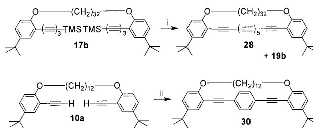
Scheme 6. Palladium-catalyzed coupling with diiodoacetylene ( 27 ) and 1,4-diiodobenzene ( 29 ) to obtain heptadiyne 28 and diethynylbenzene 30 . i) [Pd(PPh 3 ) 2 Cl 2 ], CuI, I-C≡C-I ( 27 ), NEt 3 , CH 2 Cl 2 . Yield: 28 (11%); ii) [Pd(PPh 3 ) 2 Cl 2 ], CuI, I-C 6 H 4 -I ( 29 ), NEt 3 , CHCl 3 . Yield: 30 (26%).
