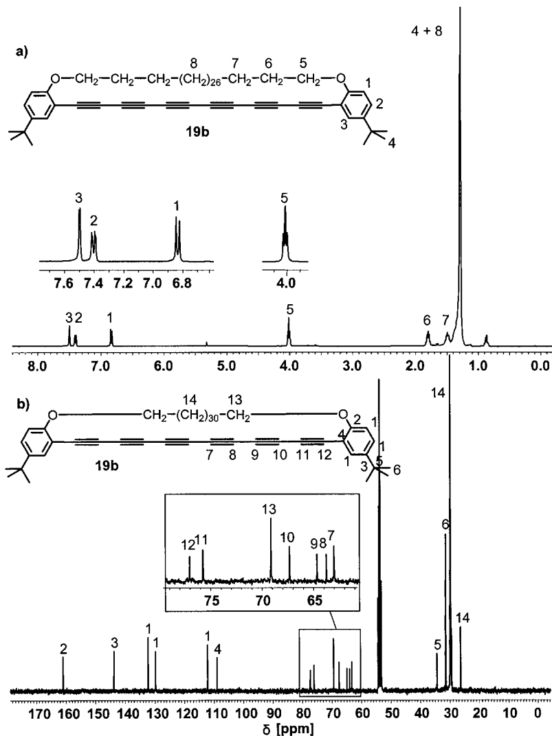
Figure 2. a) ^1\text{H} NMR spectrum (400 MHz, \text{CDCl}_3 , 25^\circ\text{C} ) and b) ^{13}\text{C} NMR (100.5 MHz, \text{CDCl}_3 , 25^\circ\text{C} ) spectrum of the 50-membered hexayne macrocycle 19b .
