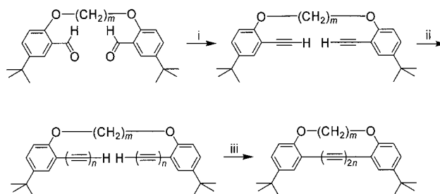
Scheme 1. Schematic representation of the preparation of oligoyne macrocycles starting with the protecting diphenyl termini. i) Formation of the acetylenic termini, ii) alkyne elongation and iii) macrocyclization.
