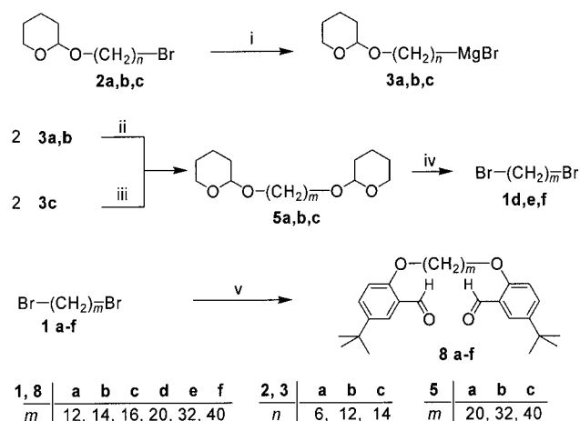
Scheme 2. Synthesis of the protecting oligomethylene-bridged diphenyl termini 8a–f . i) Mg, THF, heat; ii) I-(CH 2 ) 8 -I ( 4 ), Li_2CuCl_4 , THF, -20^\circ C ; iii) Br-(CH 2 ) 12 -Br ( 1a ), Li_2CuCl_4 , THF, -20^\circ C ; iv) 2,4,4,6-tetrabromocyclohexa-2,5-dienone ( 6 ), PPh_3 , CH_2Cl_2 ; v) 5- tert -butyl-2-hydroxybenzaldehyde ( 7 ), K_2CO_3 , DMF, 80^\circ C .
