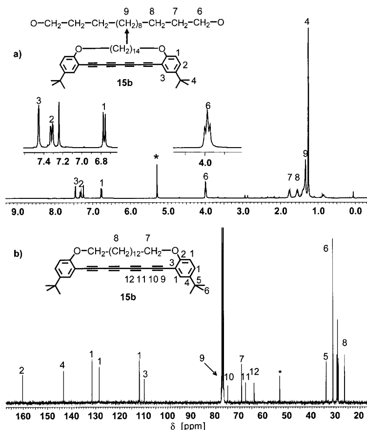
Figure 1. a) ^1\text{H} NMR spectrum (400 MHz, \text{CDCl}_3 , 25 °C) and b) ^{13}\text{C} NMR spectrum (100.5 MHz, \text{CDCl}_3 , 25 °C) of the 28-membered tetrayne macrocycle 15b (* = solvent).
