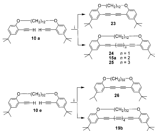
Scheme 5. Palladium-catalyzed coupling with tetraiodoethene ( 22 ). i) [Pd(PPh 3 ) 2 Cl 2 ], CuI, I 2 C=Cl 2 ( 22 ), NEt 3 , CH 3 CN, column chrom. Yields: 23 (0.4%), 24 (3.8%), 15a (1.6%), 25 (traces), 26 (5%) and 19b (3%).
